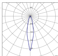
CENSER-100-16°-14W
