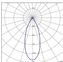
CENSER-100-38°-14W
