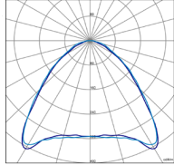
RTK/ASYM (I)-1500-115W
