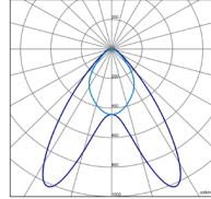
RTK/DASYM-1500-115W
